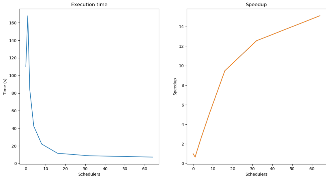
Figure 4.11: Parallel execution
