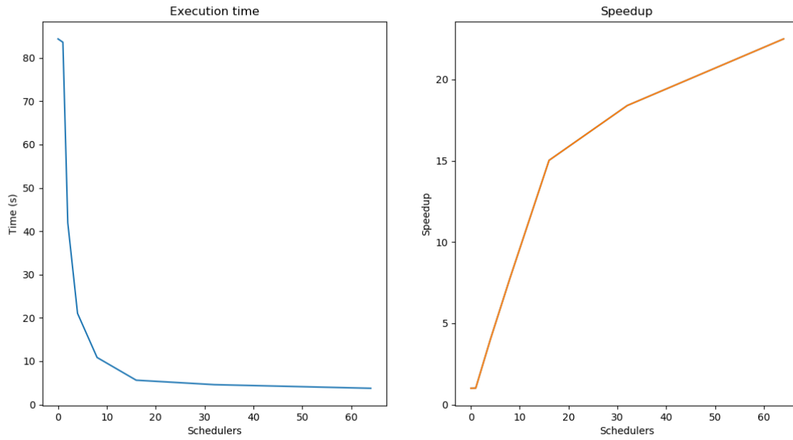
Figure 4.14: Parallel execution
