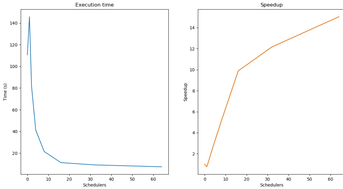
Figure 4.8: Parallel execution
