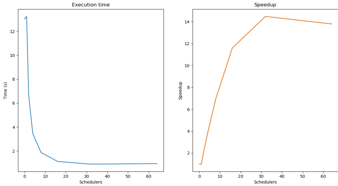
Figure 4.5: Parallel execution
